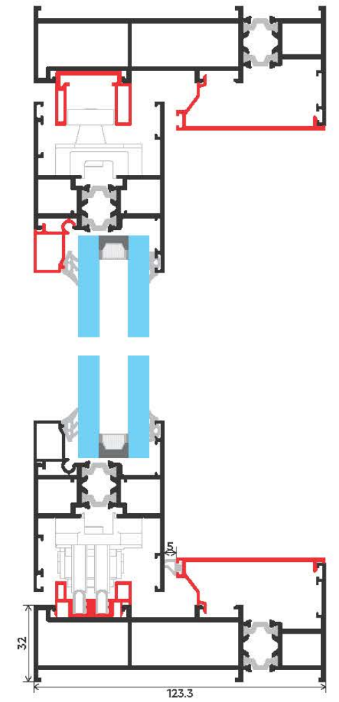
Locking Position
