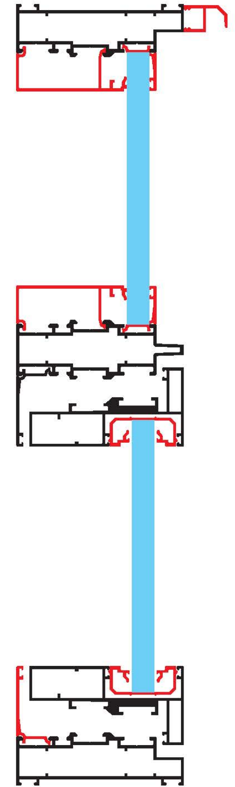
SGU Assembly
