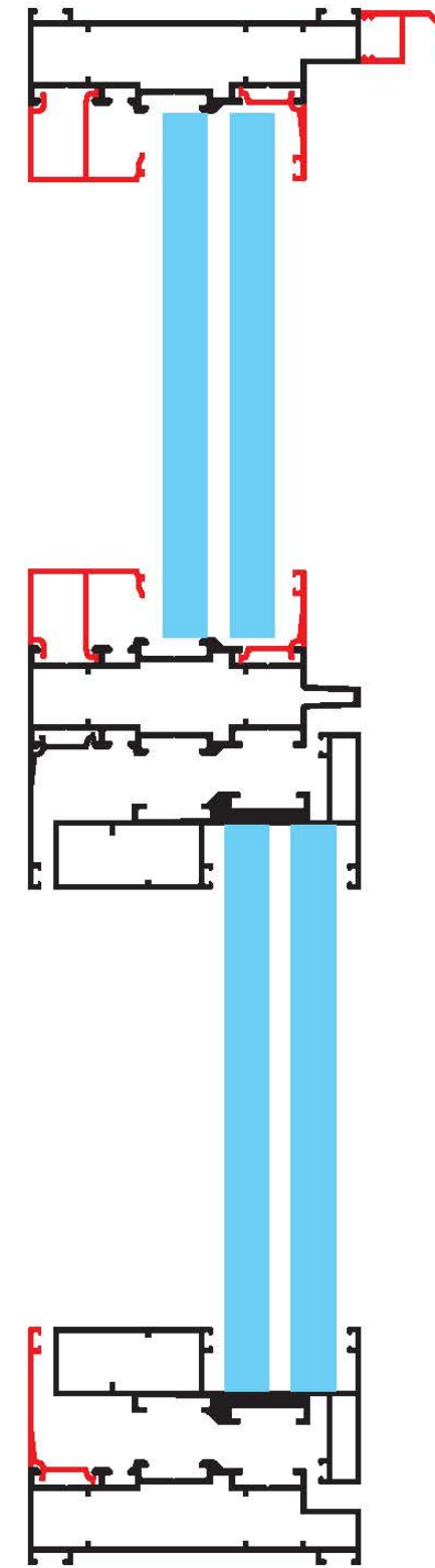
DGU Assembly
