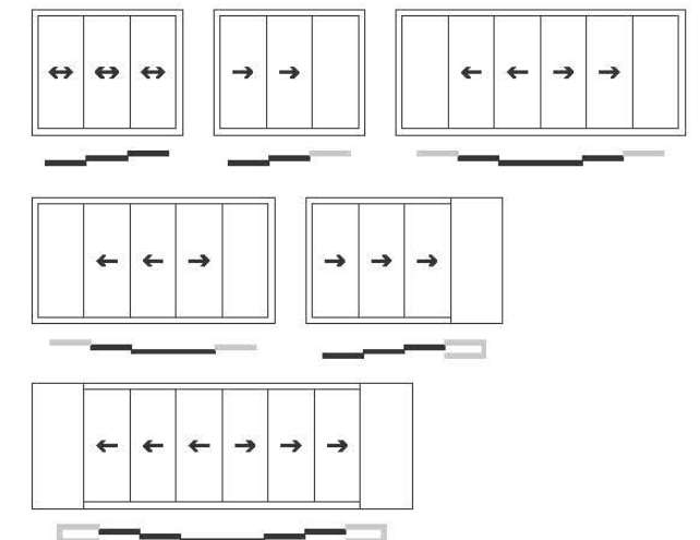
3 Track
