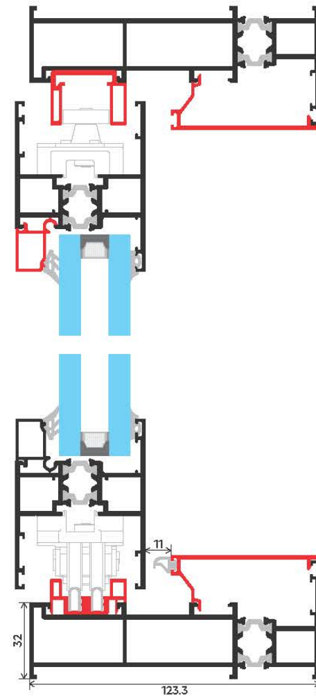
Sliding Position
